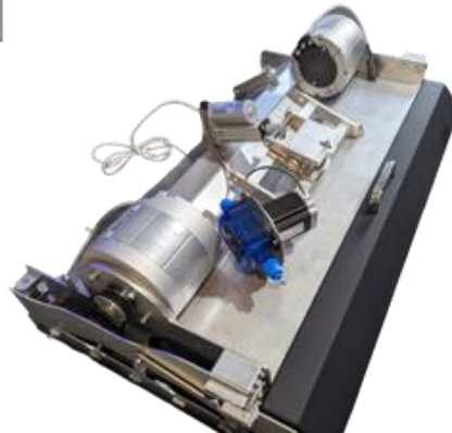
Stainless steel brush deck ANTI-RUST
